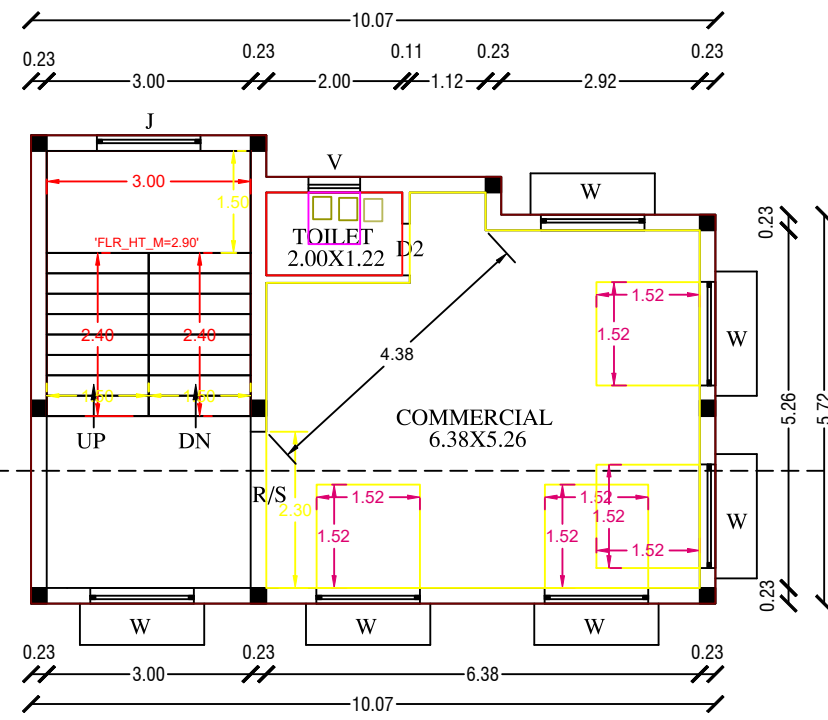
FIRST FLOOR PLAN (COM.)
