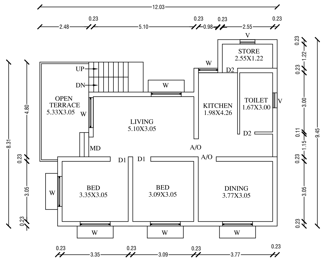
FIRST FLOOR PLAN DEMOLISHION PLAN
