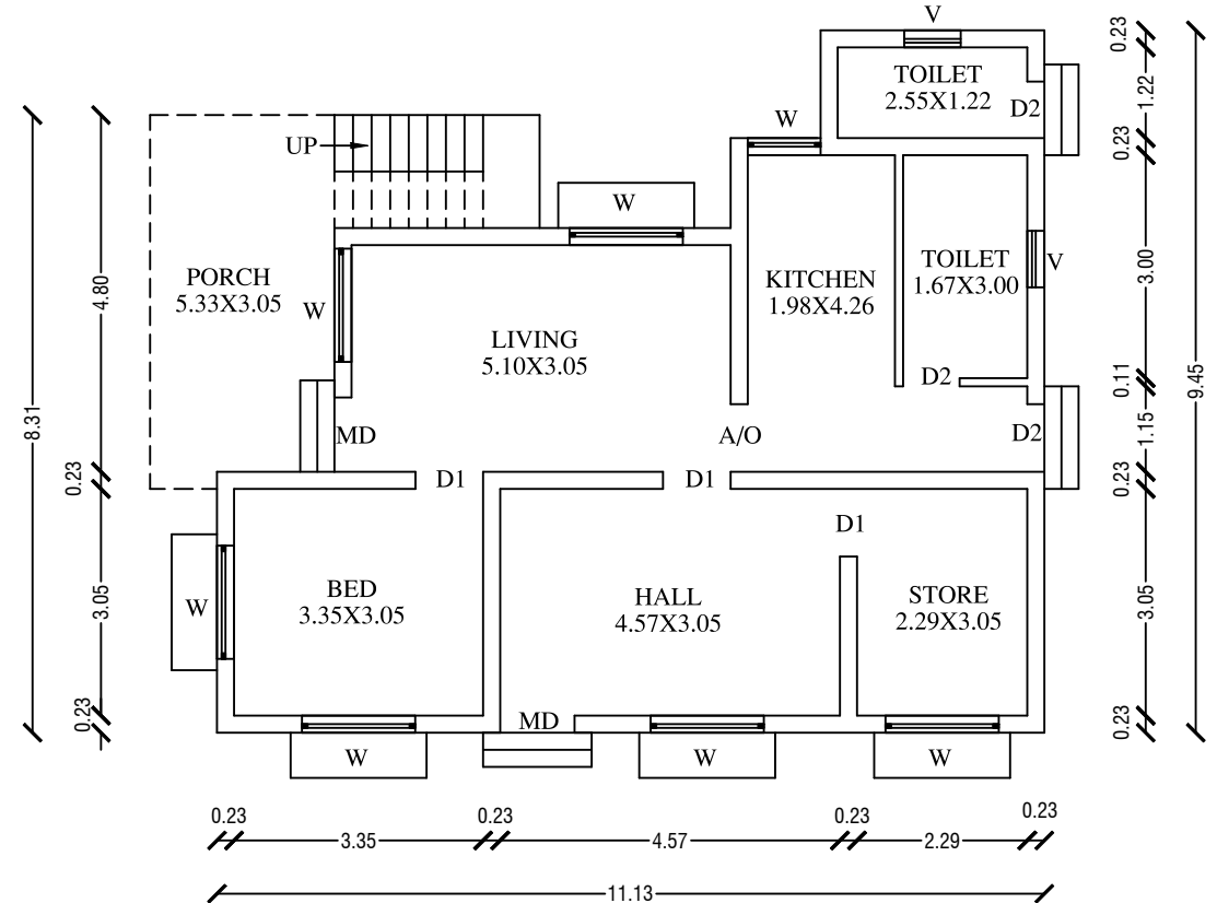
GROUND FLOOR PLAN DEMOLISHION PLAN
