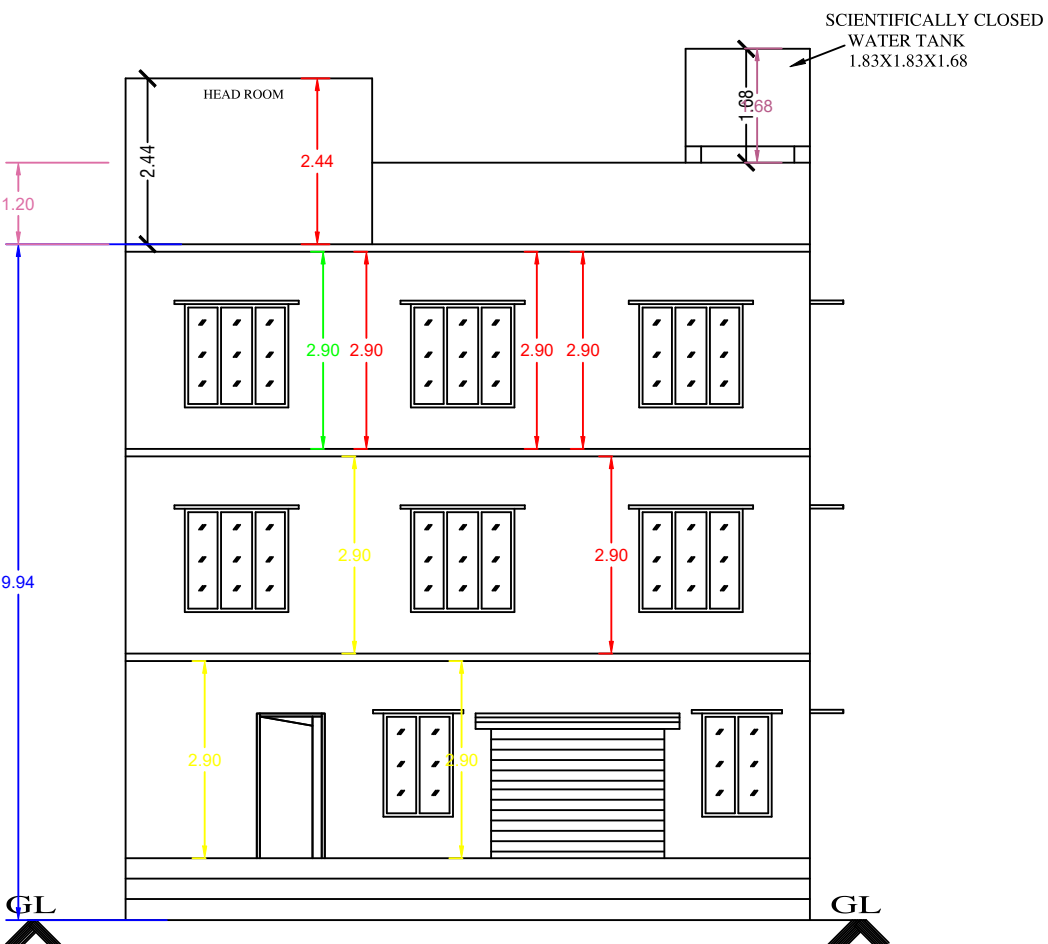
FRONT ELEVATION
