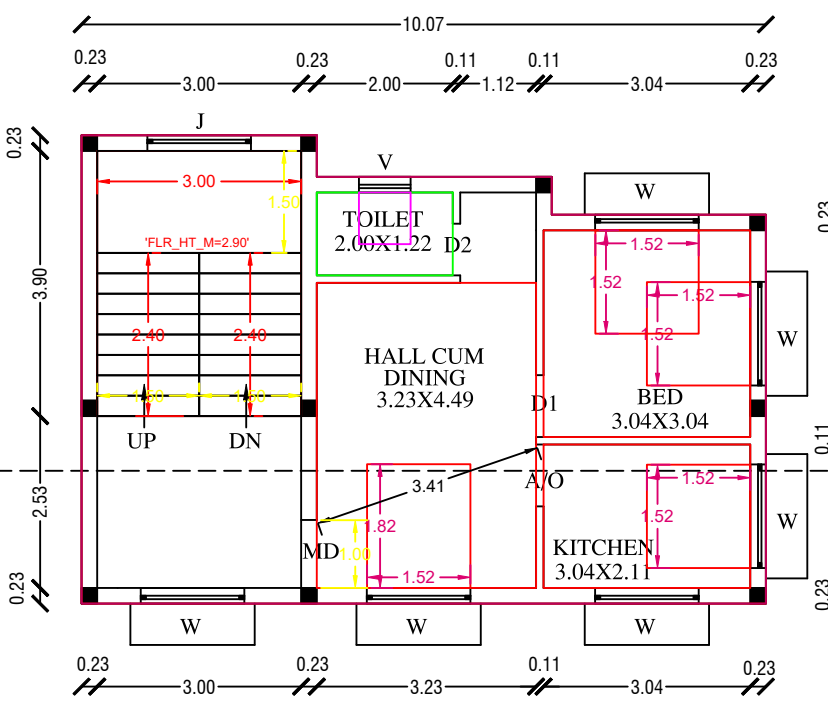
SECOND FLOOR PLAN (RES.)
