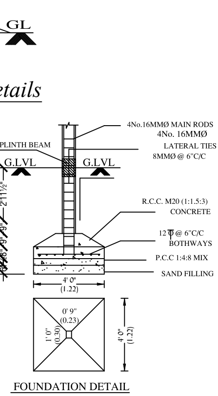
FOUNDATION DETAIL (SCALE: 1:30)
