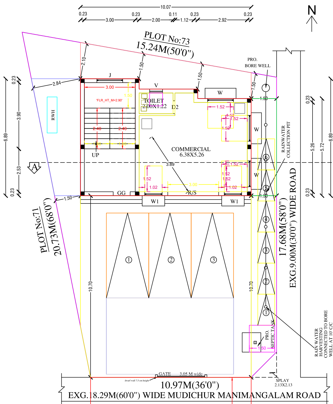
SITE PLAN CUM GROUND FLOOR PLAN (COM.)
