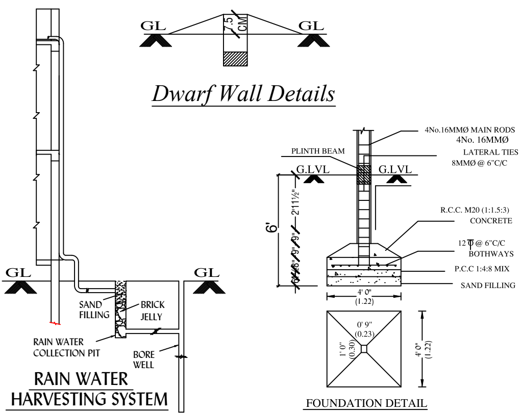
FOUNDATION DETAIL (SCALE: 1:30)
