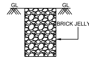
PERCOLATION PIT
