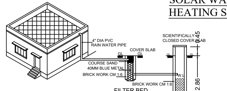
PROPOSED RAIN WATER SYSTEM WITH WELL DETAIL
