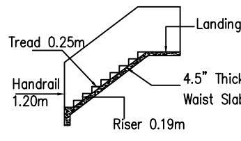
STAIRCASE DETAIL
