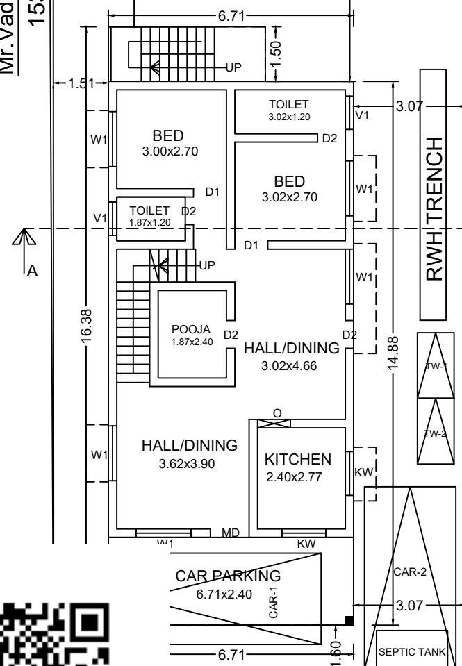
37'-0" [11.28M] 18'-0" WIDE ROAD RO.GROUND FLOOR PLAN
