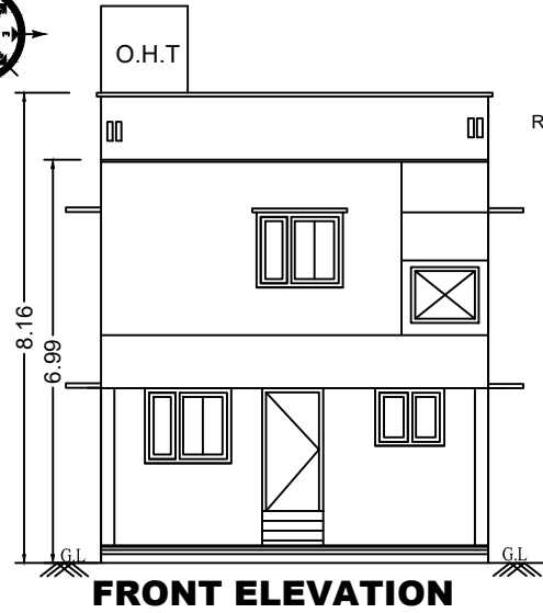
FRONT ELEVATION
