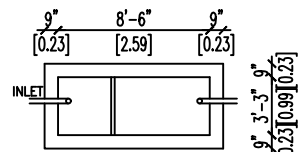
DETAILS OF SEPTIC TANK
