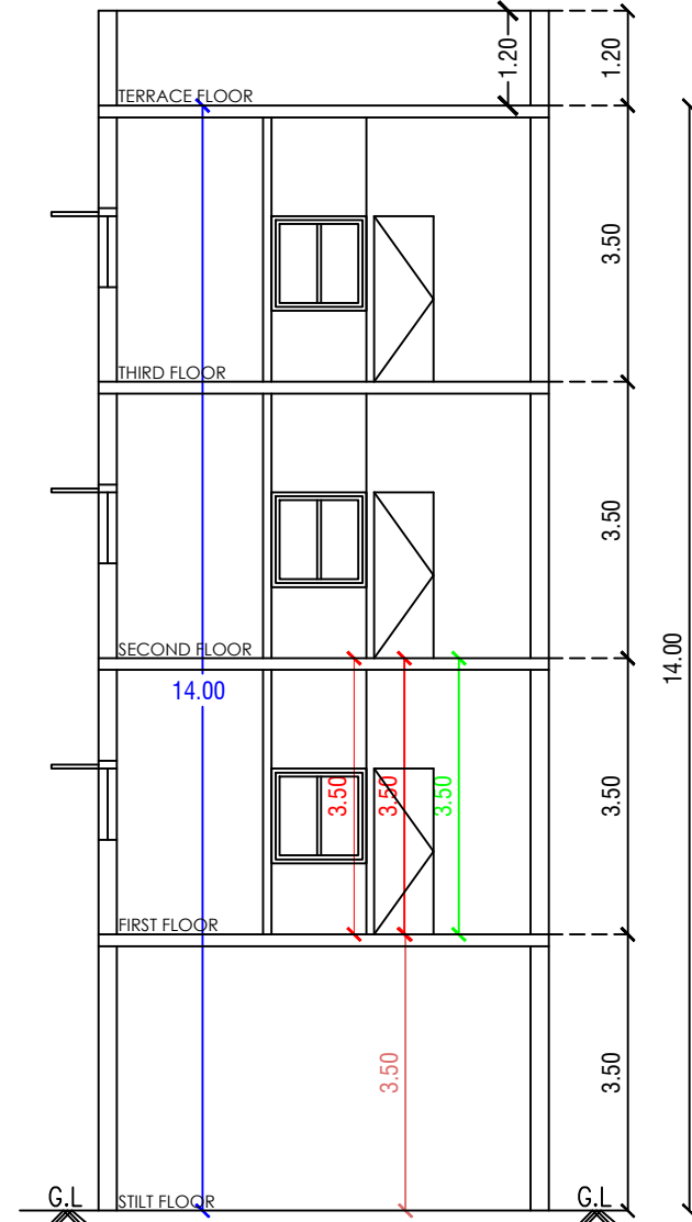
SECTION 'X-X'
