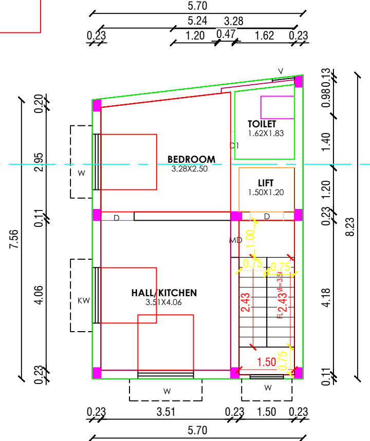
1st, 2nd & 3rd FLOOR PLAN (PROPOSED)
