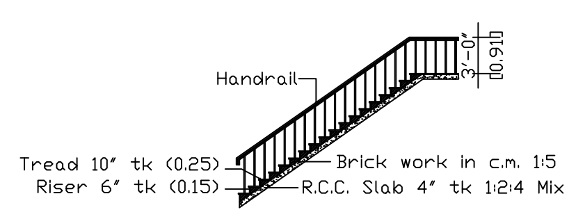
Staircase Details
