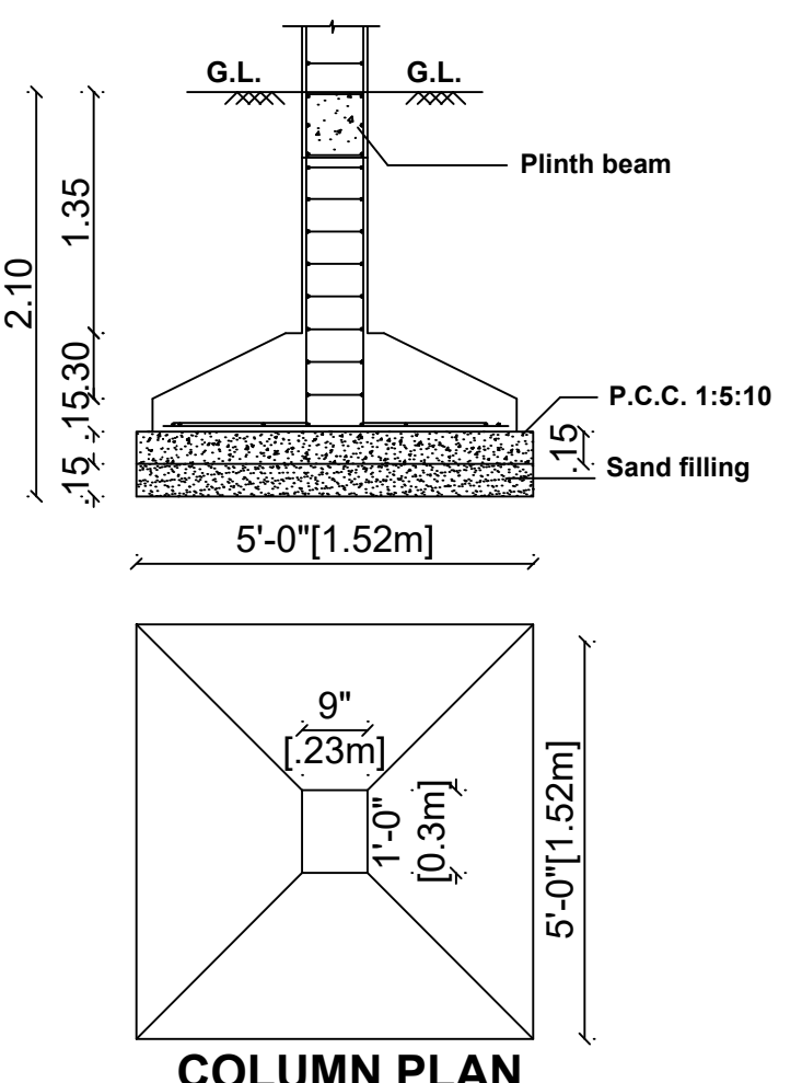
COLUMN PLAN SIZE:- 0.23x0.30 m TYPICAL FOUNDATION DETAIL Footing Detail
