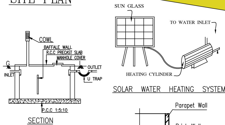
SECTION
