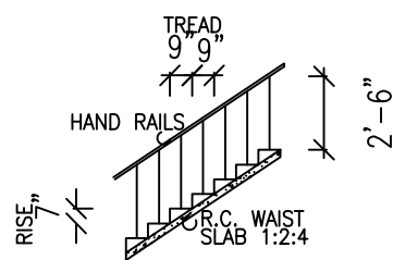
STAIRCASE DETAILS
