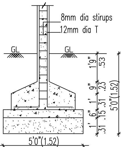
COLUMN FOUNDATION DETAIL
