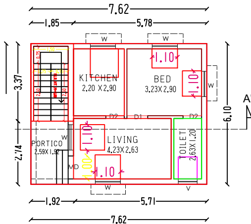
GROUND FLOOR SCALE 1:100
