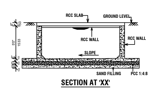
RWHTRENCH
