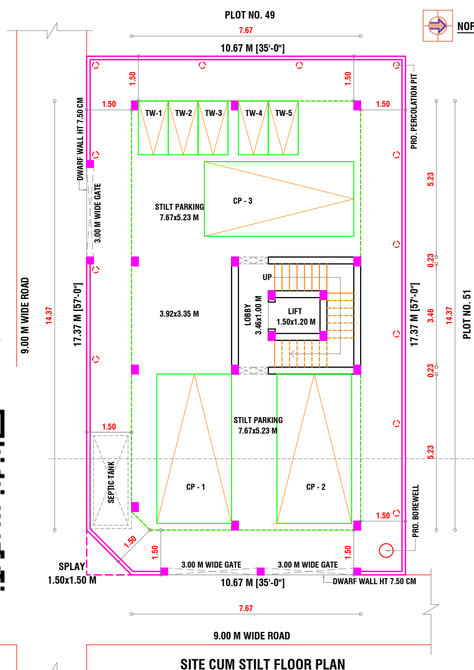
SITE CUM STILT FLOOR PLAN
