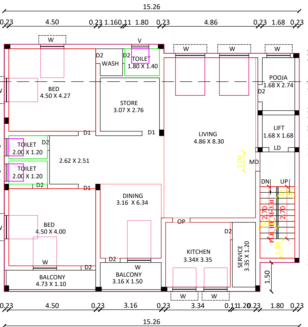
PRO.SECOND FLOOR PLAN
