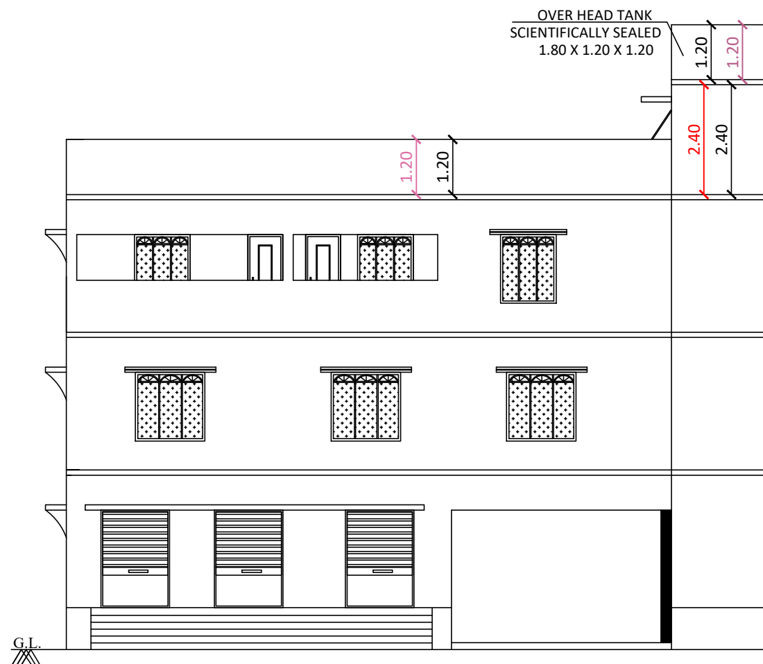
FRONT ELEVATION
