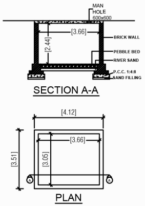
TYPICAL SUMP DETAIL FOR RAIN WATER HARVESTING FROM TERRACE FLOOR
