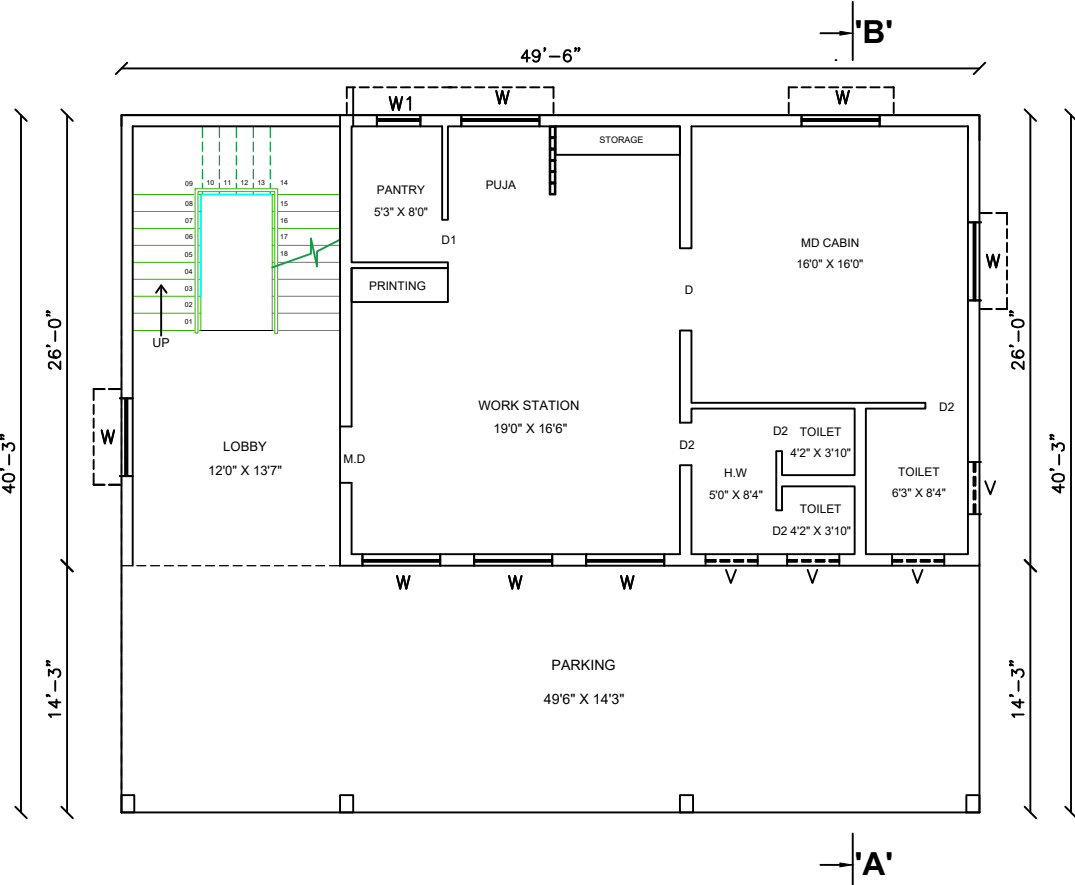
FLOOR PLAN
