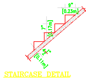
STAIRCASE DETAIL
