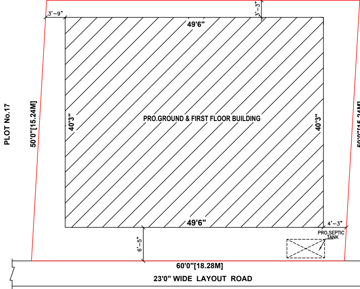
SITE PLAN
