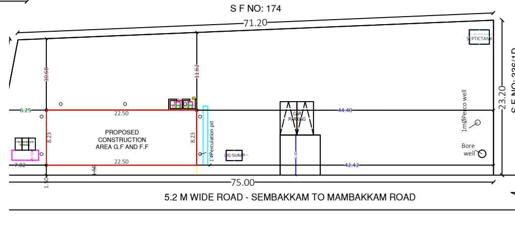
SITE PLAN SCALE 1:50
