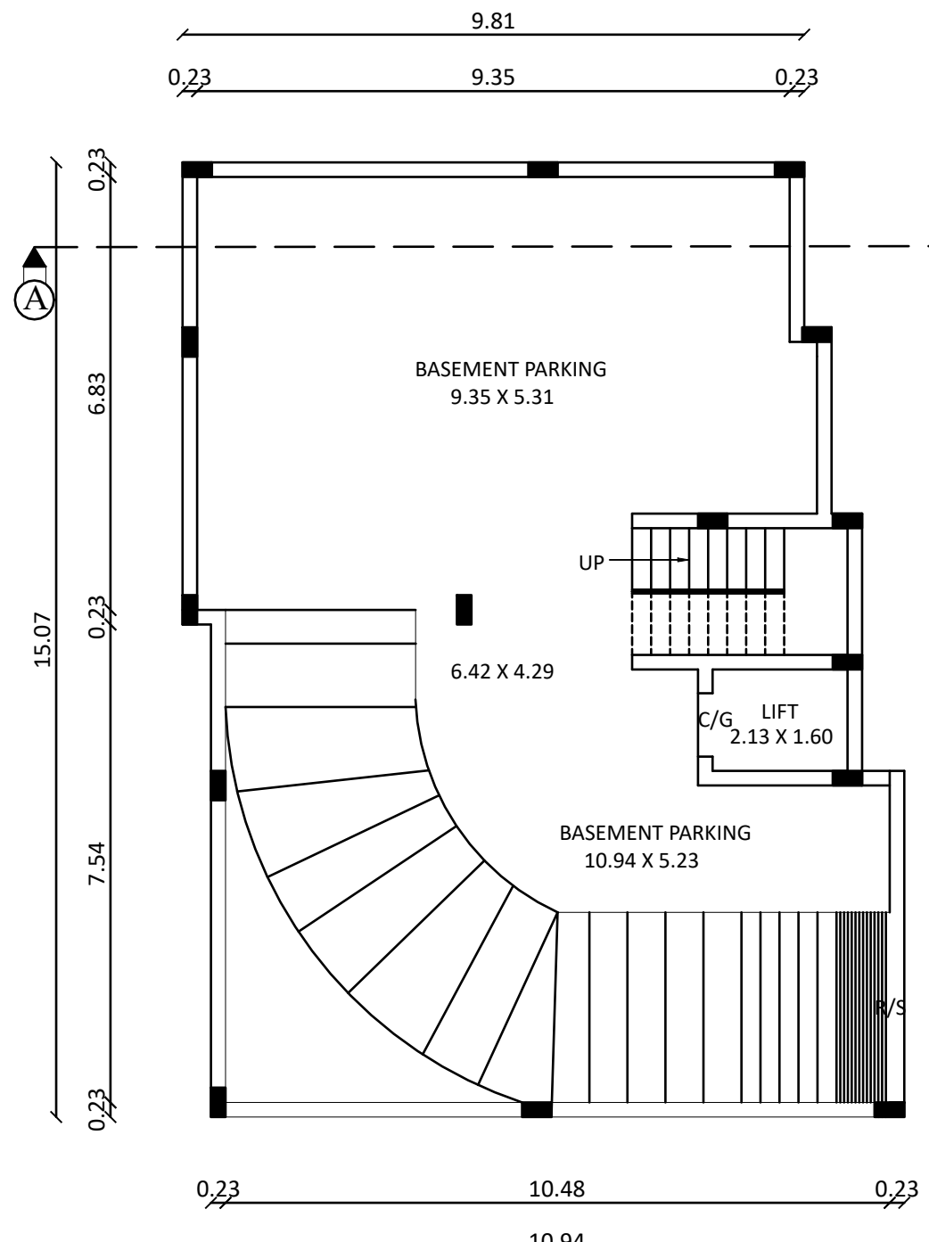
PRO.BASEMENT FLOOR PLAN
