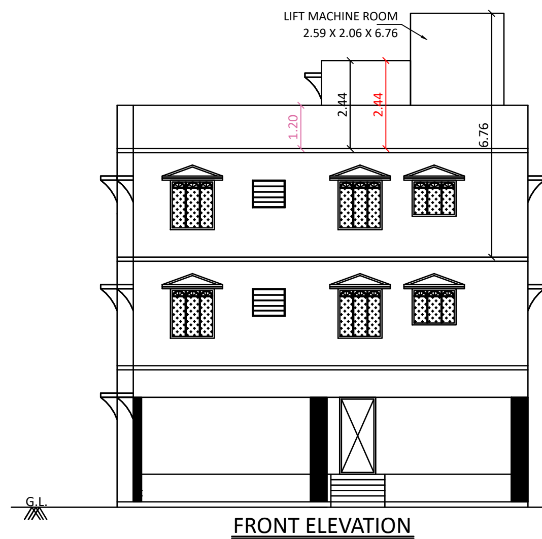
FRONT ELEVATION
