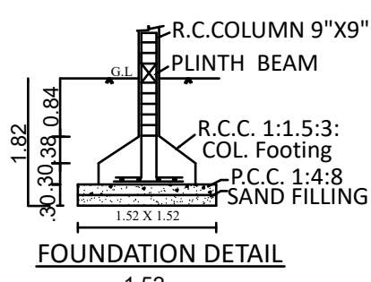
FOUNDATION DETAIL
