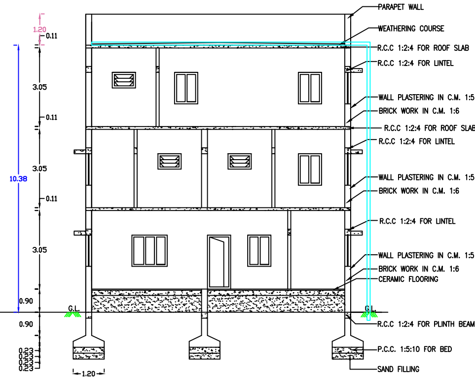
SECTION ON "R-C"
