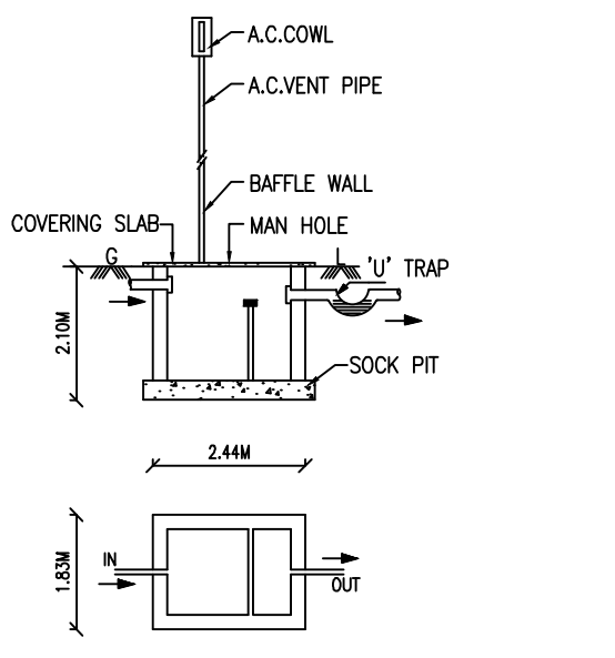
SEPTIC TANK
