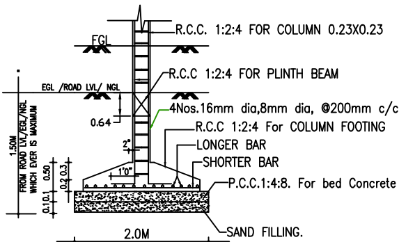
FOUNDATION DETAILS
