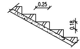
STAIRS DETAILS
