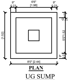
PLAN UG SUMP
