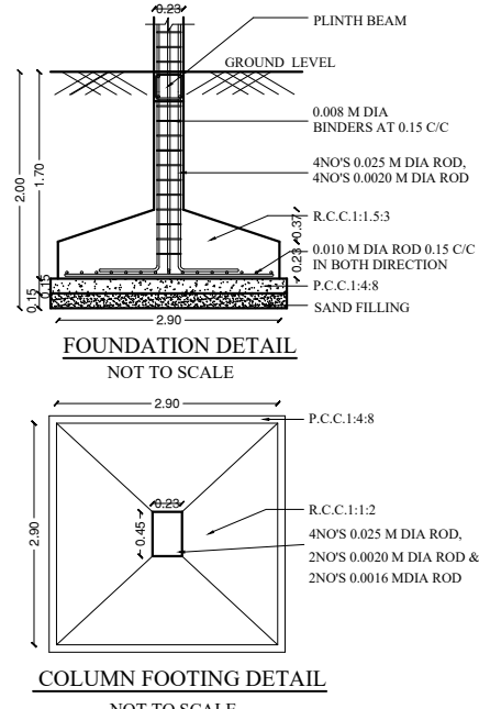
COLUMN FOOTING DETAIL NOT TO SCALE
