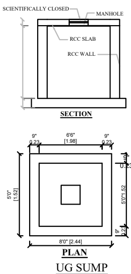
PLAN UG SUMP
