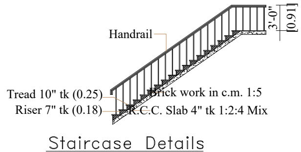
Staircase Details
