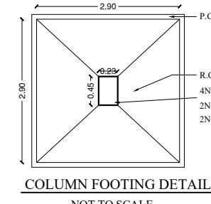
COLUMN FOOTING DETAIL NOT TO SCALE
