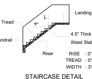
STAIRCASE DETAIL
