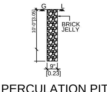
PERCOLATION PIT
