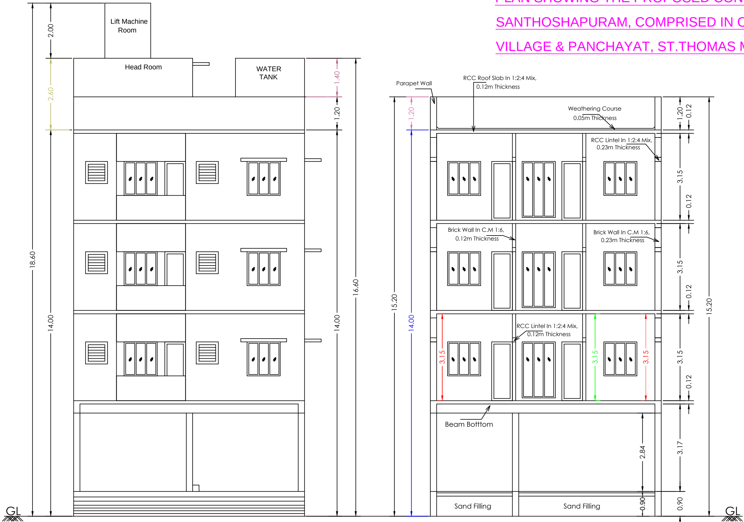
FRONT ELEVATION.
