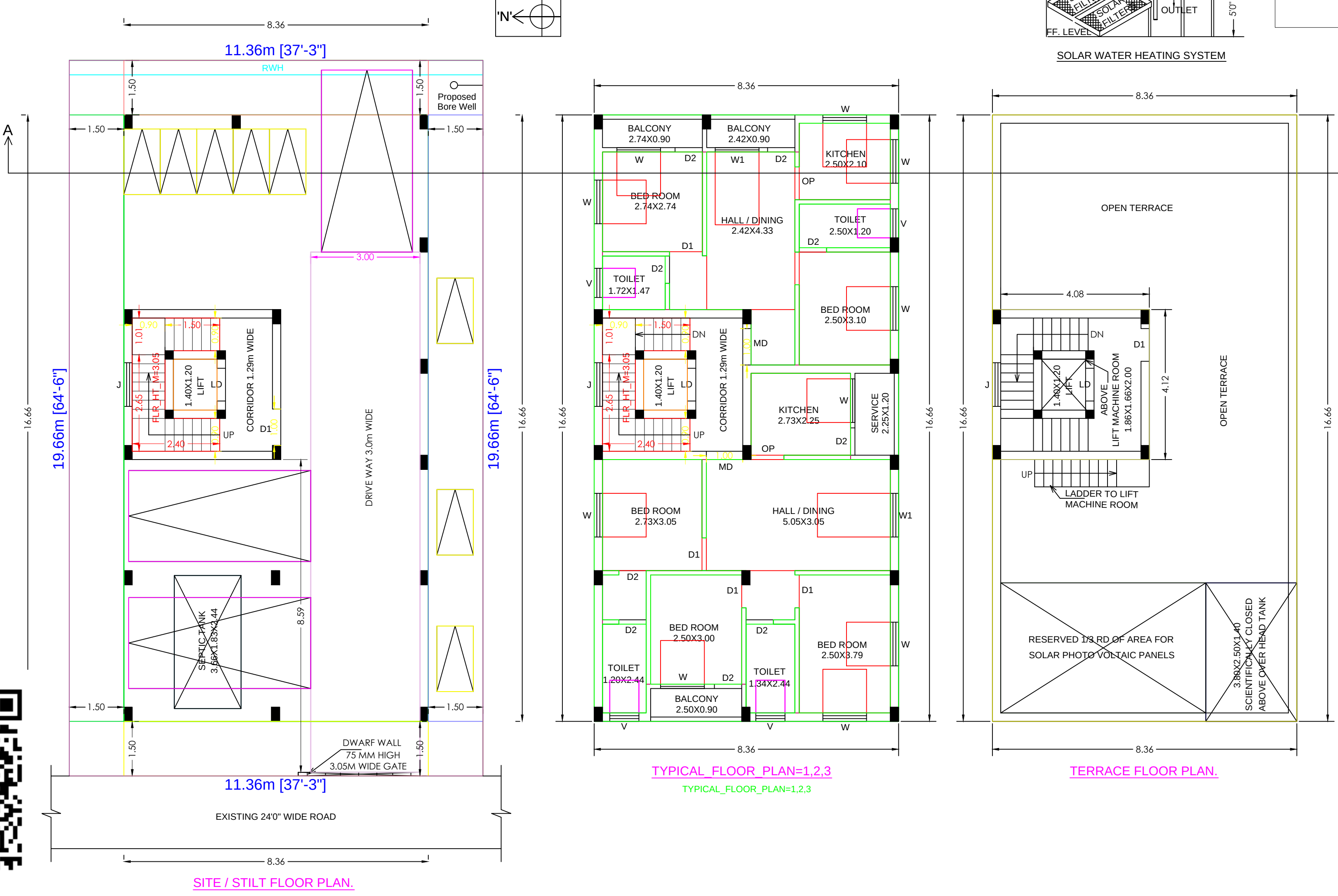
SITE / STILT FLOOR PLAN.
