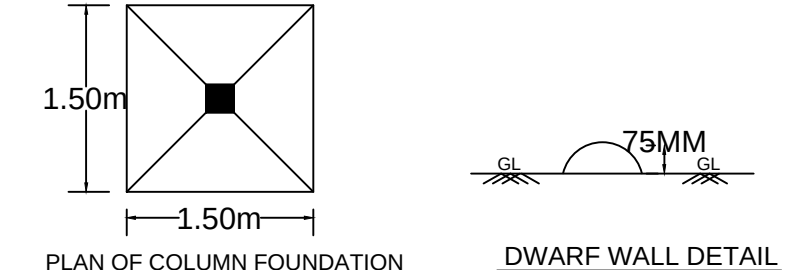
PLAN OF COLUMN FOUNDATION
