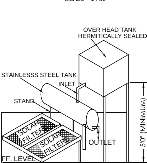
SOLAR WATER HEATING SYSTEM
