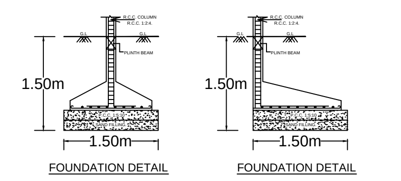
FOUNDATION DETAIL
