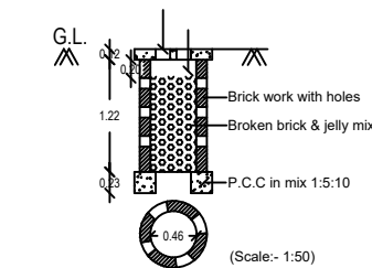
RAIN WATER COLLECTION WELL
