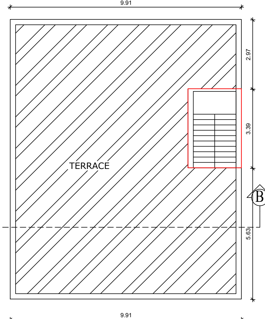
PRO.TERRACE & HEADROOM
