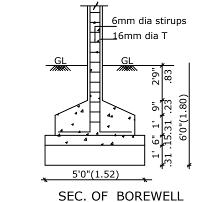
SEC. OF BOREWELL
