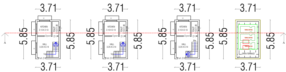
PRO GROUND FLOOR PLAN
