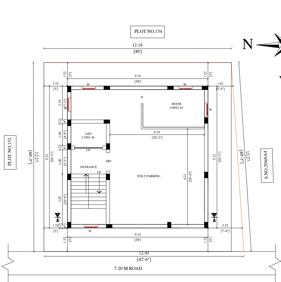
PRO.SITE CUM STILT FLOOR PLAN
