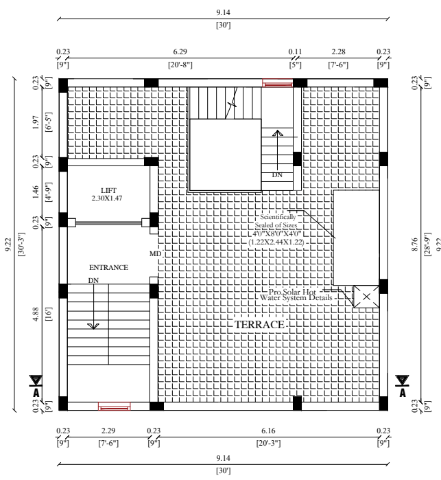
PRO.TERRACE FLOOR PLAN
