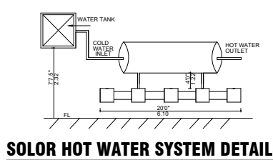
SOLAR HOT WATER SYSTEM DETAILS
