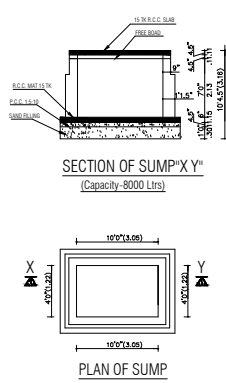
SECTION OF SUMP 'X-Y'
