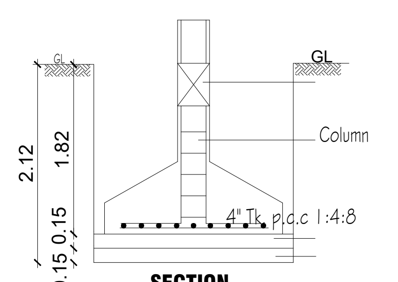
PLAN FOUNDATION DETAIL
