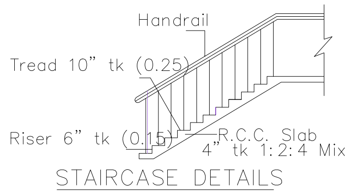
STAIRCASE DETAILS
