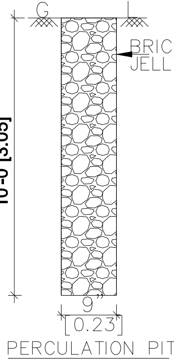
PERCOLATION PIT
