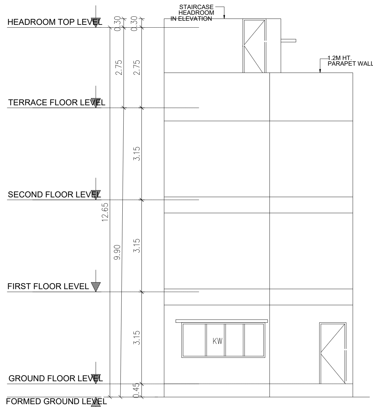
FRONT ELEVATION
