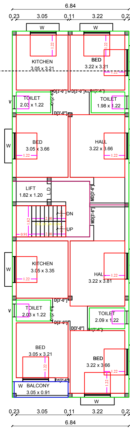
THIRD FLOOR PLAN
