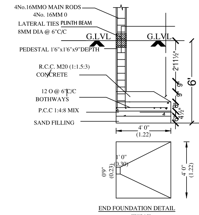
END FOUNDATION DETAIL (SCALE 1:30)
