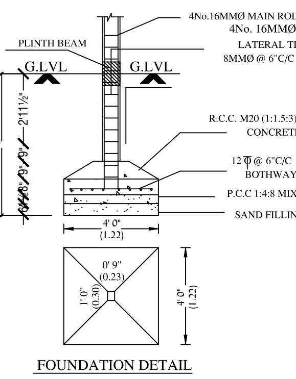
FOUNDATION DETAIL (SCALE 1:30)
