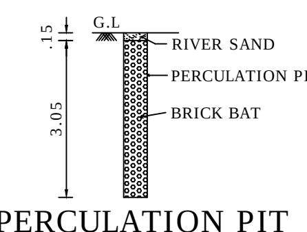
PERCULATION PIT
