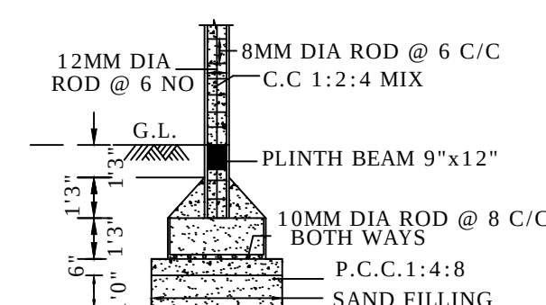
[1.22x1.22] RUN THROUGH COLUMN FOUNDATION SCALE 1" = 4'0" (1:50)
