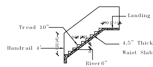
STAIRCASE DETAIL
