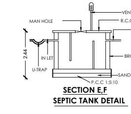
SECTION E.E SEPTIC TANK DETAIL
