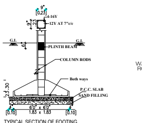
TYPICAL SECTION OF FOOTING
