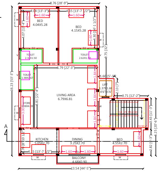
THIRD FLOOR
