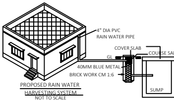
RAIN WATER PERCO WELL
