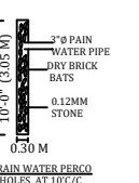
RAIN WATER PERCO HOLES
