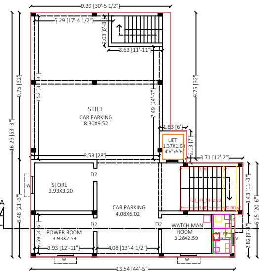
STILT FLOOR
