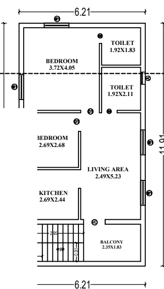
ST FLOOR PLAN
