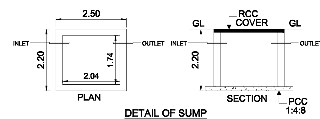
DETAIL OF SUMP
