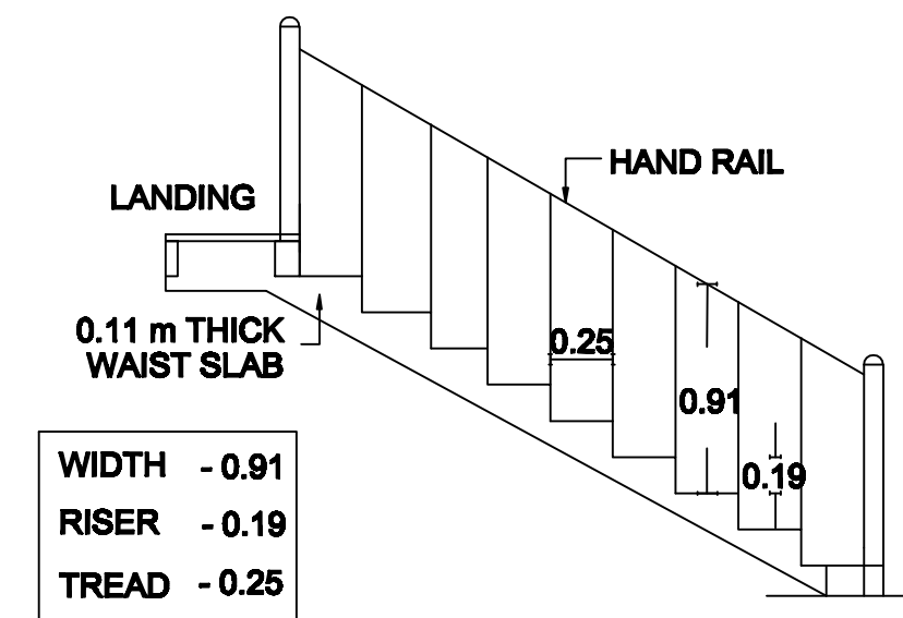
STAIRCASE DETAIL
