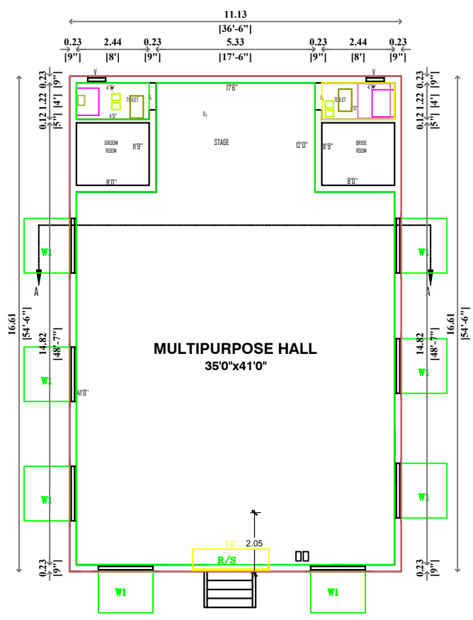
PROPOSED GROUND FLOOR PLAN (COMMERCIAL)
