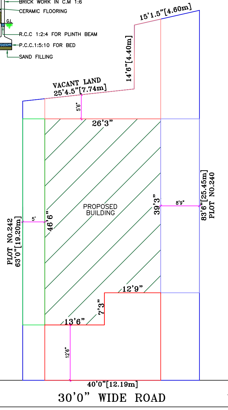
SITE PLAN
