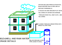
Borewell and Rain Water Storage Details
