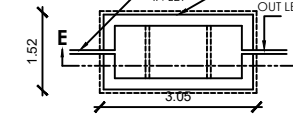
PLAN PLAN OF SEPTIC TANK
