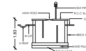
SECTION E-E SEPTIC TANK DETAIL
