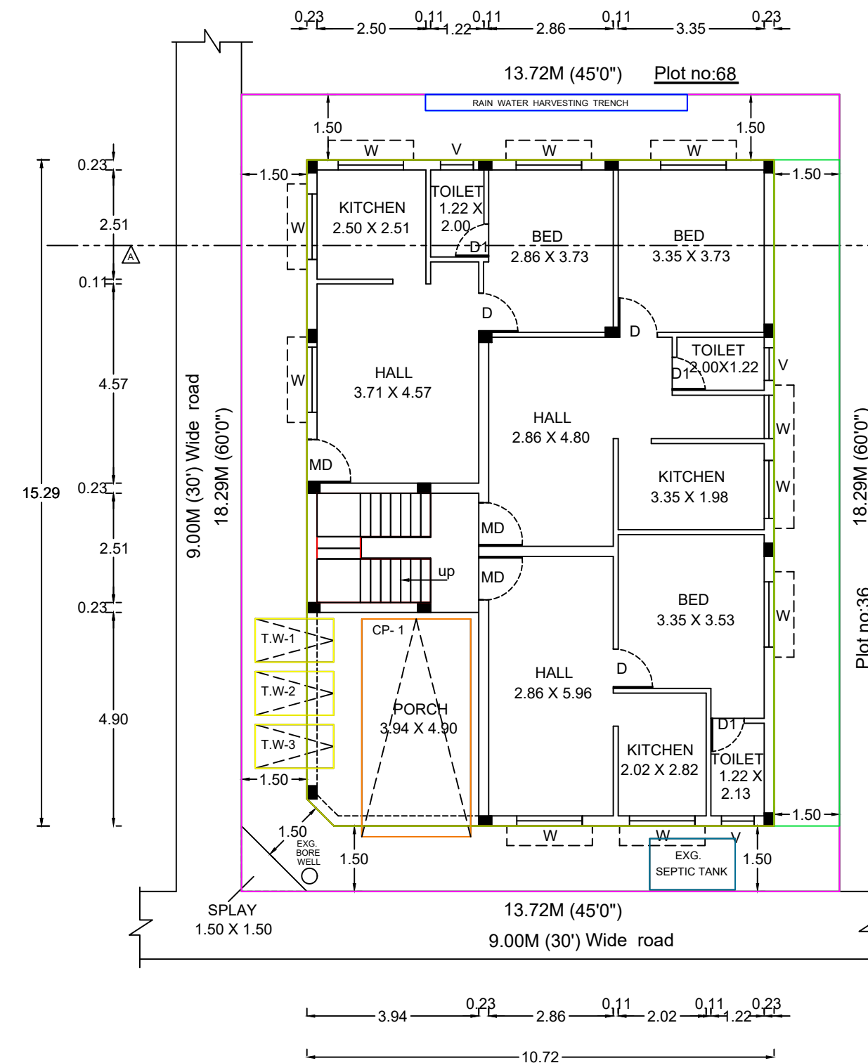
SITE CUM GROUND FLOOR PLAN ( EXISTING )
