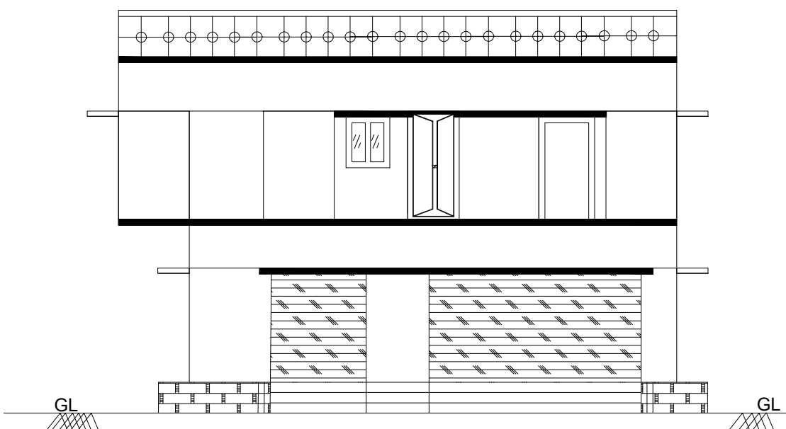
FRONT ELEVATION
