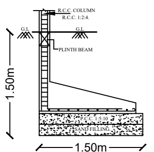
FOUNDATION DETAIL
