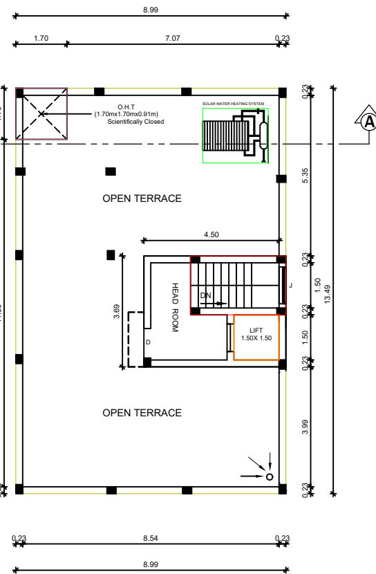
TERRACE PLAN
