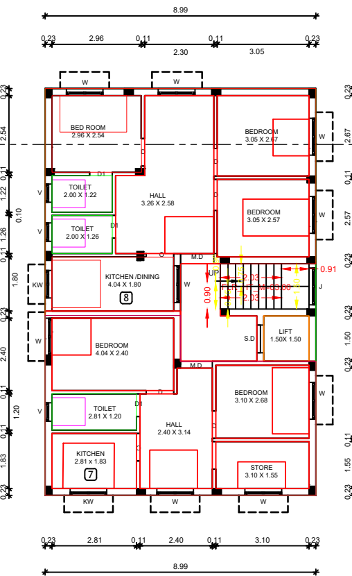
PRO. THIRD FLOOR PLAN
