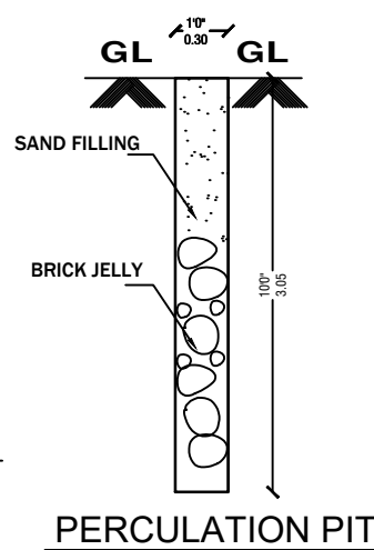
PERCOLATION PIT
