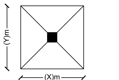
PLAN OF COLUMN FOUNDATION
