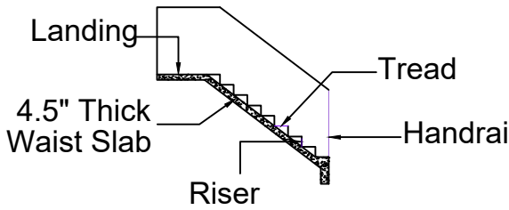
STAIRCASE DETAIL
