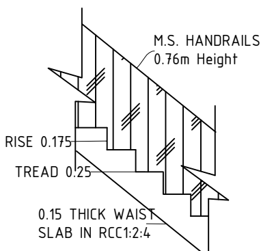
STAIRCASE DETAILS
