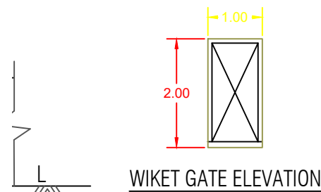
WIKET GATE ELEVATION
