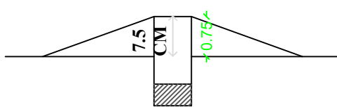
DWARF WALL DETAILS
