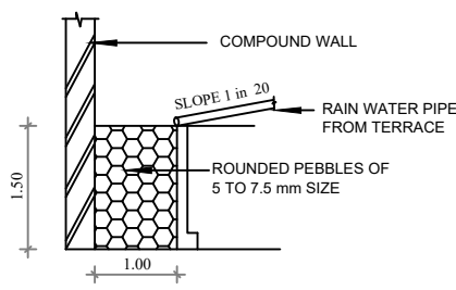
RAIN WATER CONSERVATION TRENCH DETAILS
