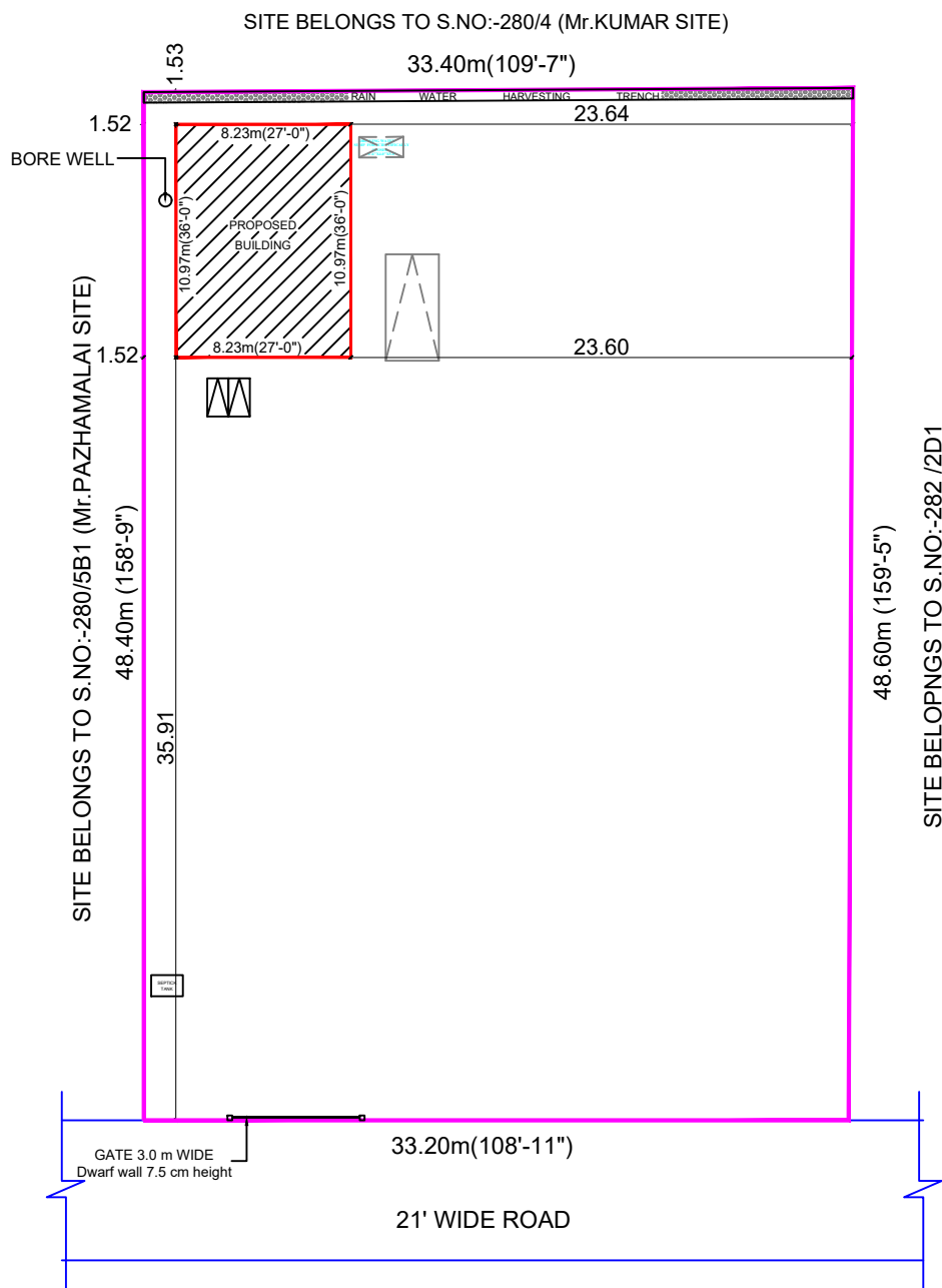
SITE PLAN (1:400) PROPOSED
