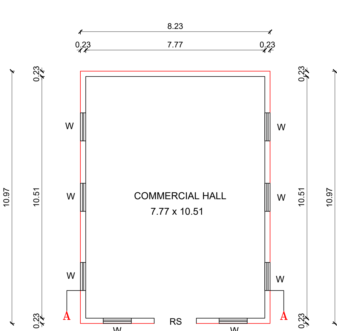
GROUND FLOOR PLAN PROPOSED
