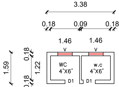
PROPOSED TOILET PLAN
