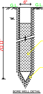
BORE WELL DETAIL
