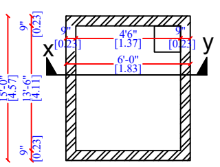
U.G.SUMP-PLAN HERMITICALLY SEALED
