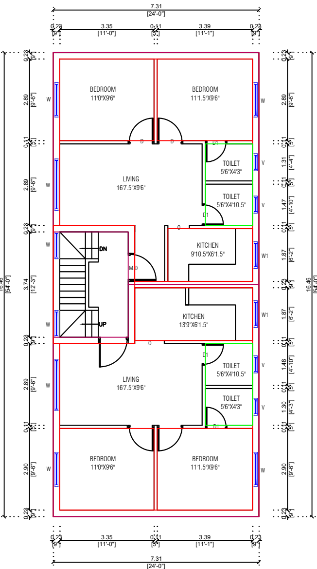
PRO.SECOND FLOOR PLAN
