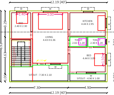
SECOND FLOOR SCALE 1:100
