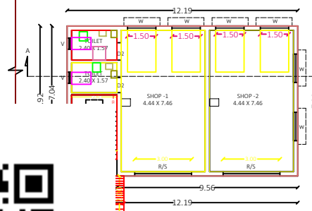
GROUND FLOOR SCALE 1:100
