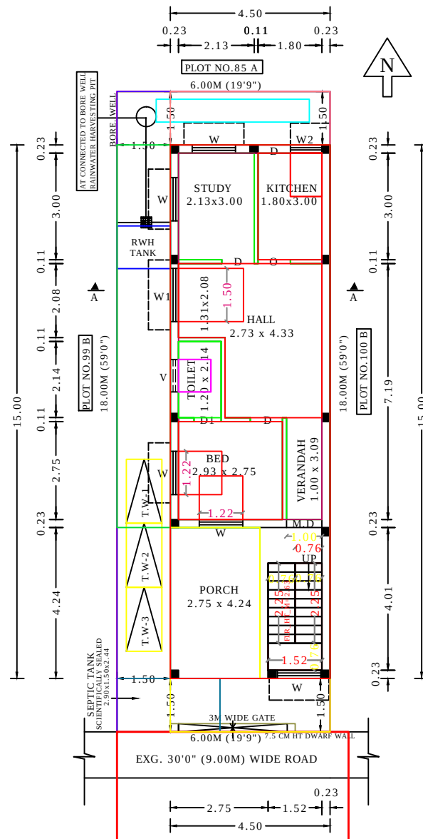
CUM ADDITIONAL GROUND FLOOR PLAN
