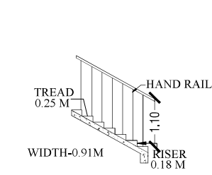
STAIRCASE DETAILS
