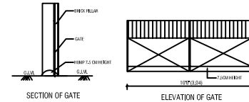
SECTION OF GATE
