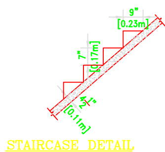
STAIRCASE DETAIL
