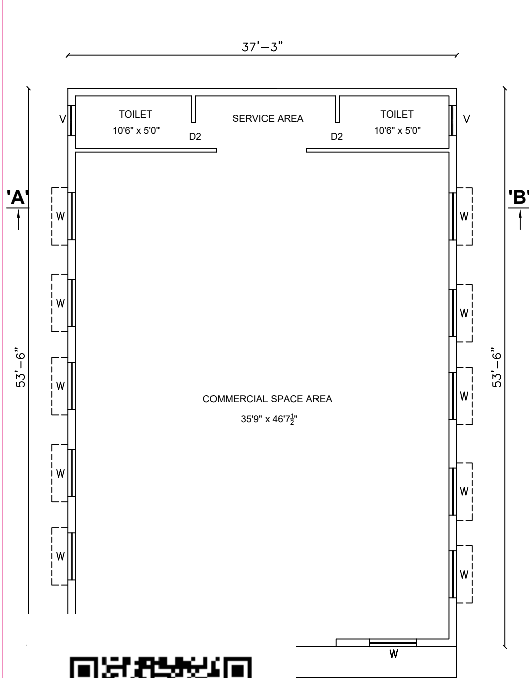
FLOOR PLAN
