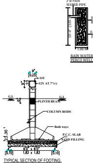
TYPICAL SECTION OF FOOTING
