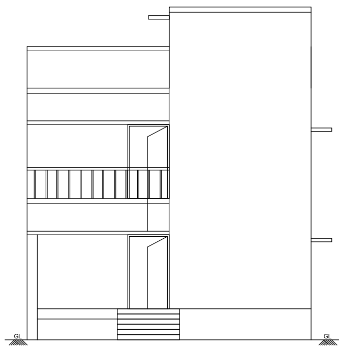
NORTH SIDE ELEVATION
