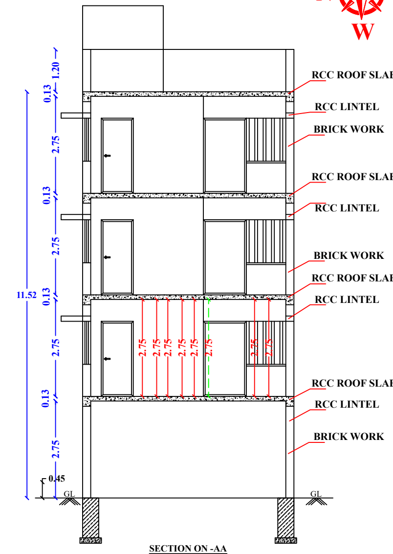
SECTION ON-AA
