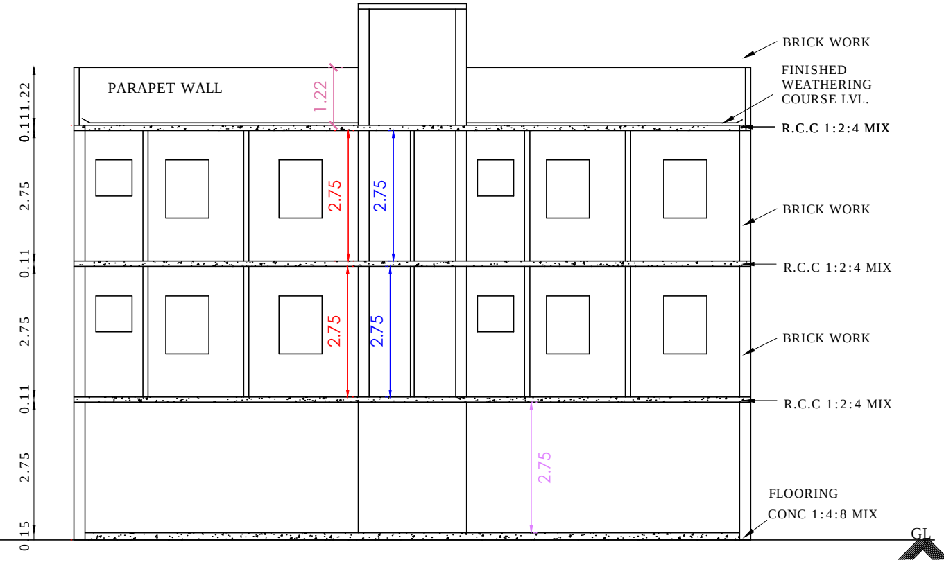
SECTION 'A-A'
