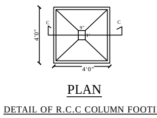
PLAN DETAIL OF R.C.C. COLUMN FOOTING
