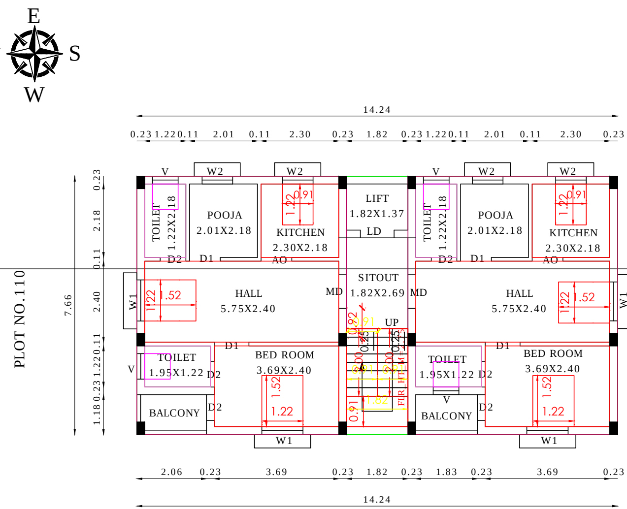
TYPICAL 1st & 2nd FLOOR PLAN
