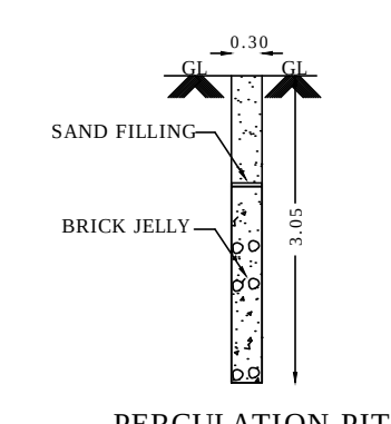
PERCOLATION PIT
