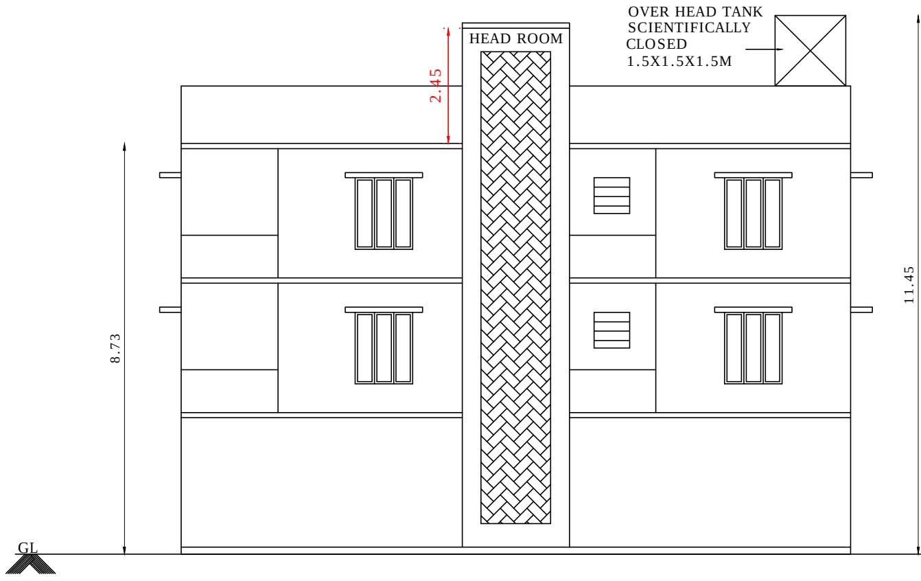
FRONT ELEVATION
