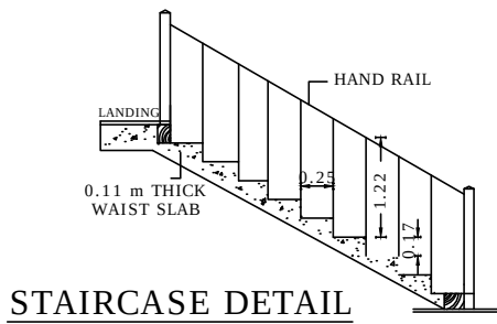
STAIRCASE DETAIL
