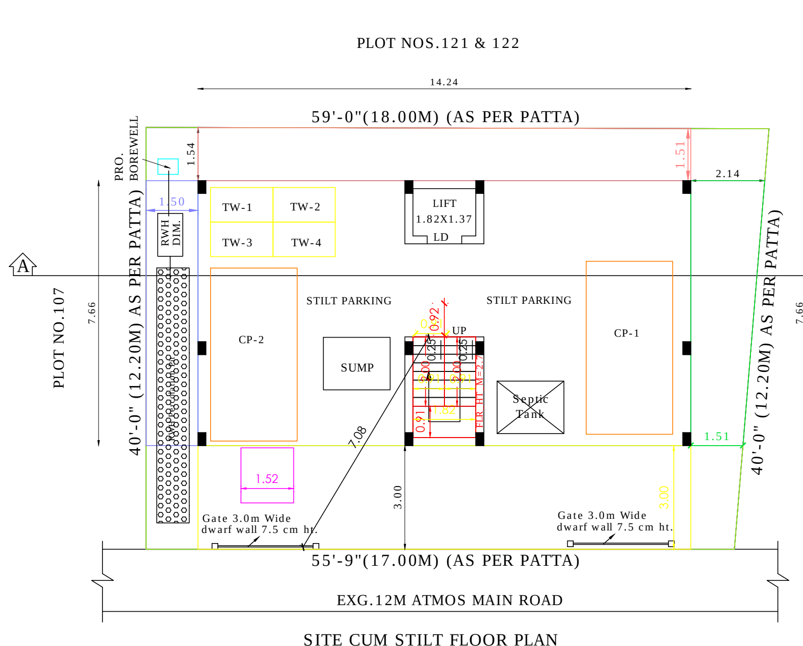
SITE CUM STILT FLOOR PLAN
