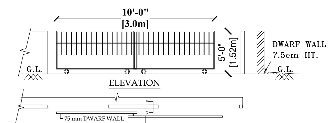
COMPOUND WALL & GATE DETAIL
