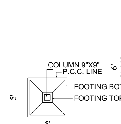
PLAN OF FOOTING
