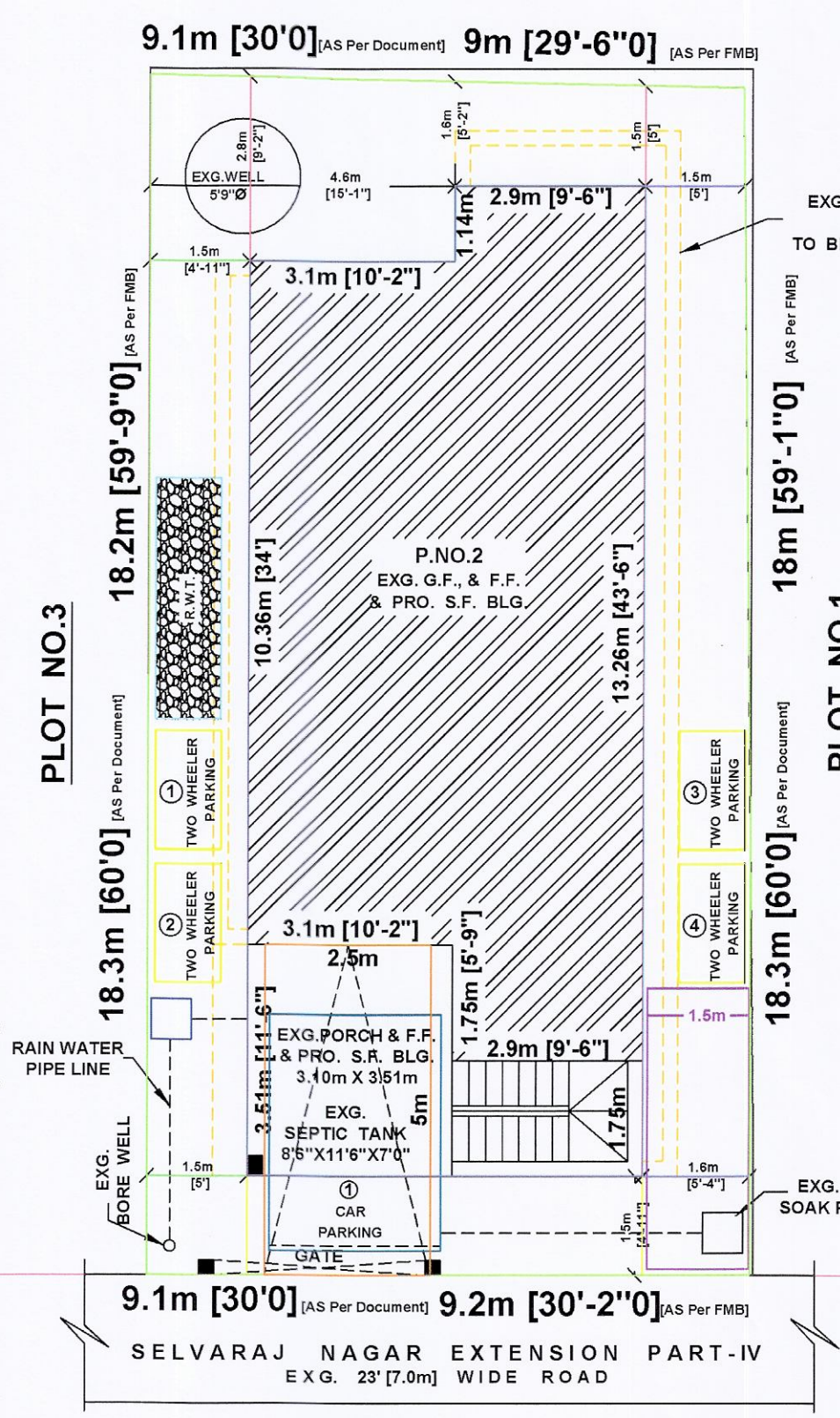
SITE PLAN
