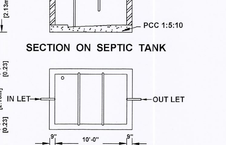
PLAN OF SEPTIC TANK (SCALE 1:50)
