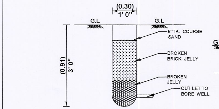
PERCOLATION PIT (NOT TO SCALE)
