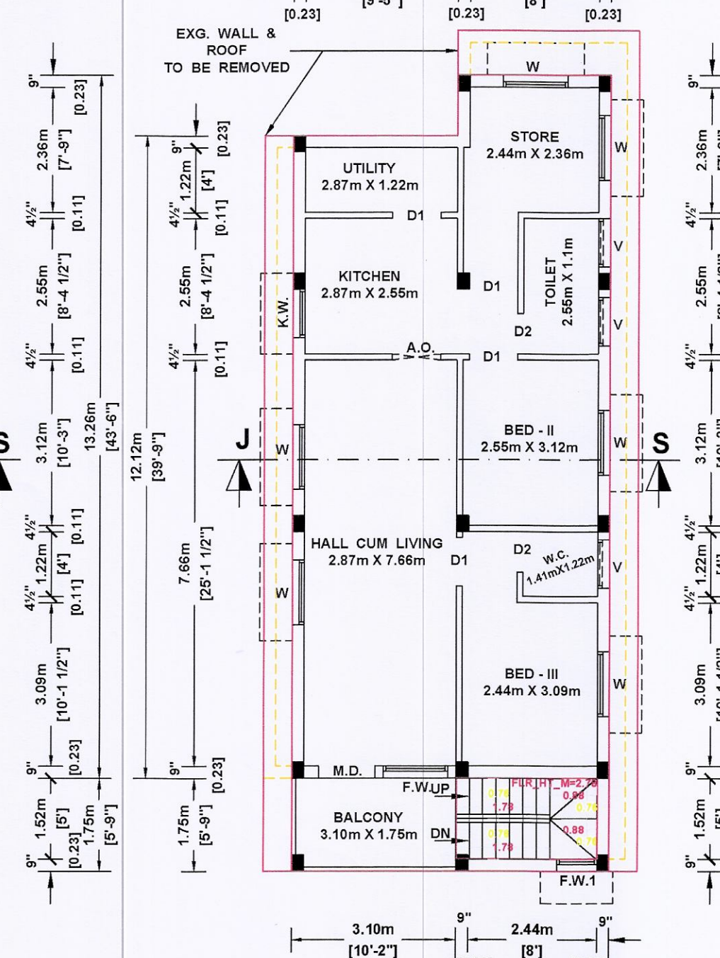
EXG. FIRST FLOOR PLAN
