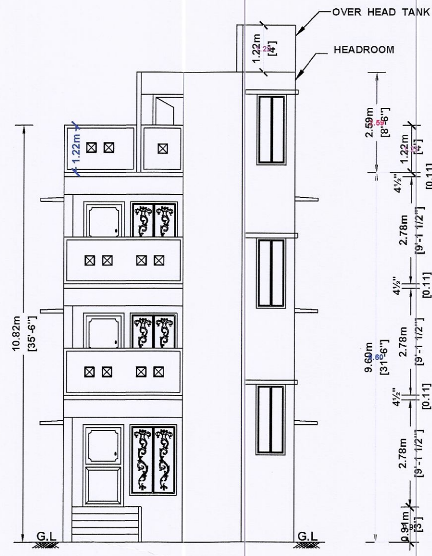
FRONT ELEVATION
