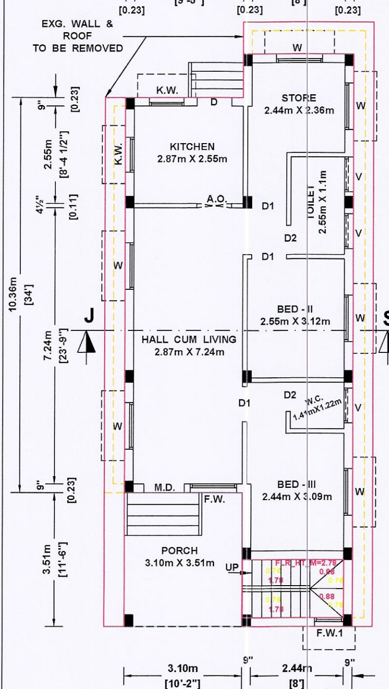
EXG. GROUND FLOOR PLAN
