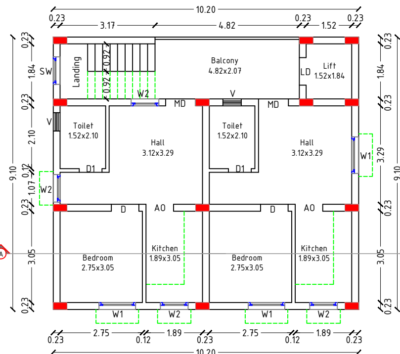
TYPICAL FLOOR PLAN SECOND AND THIRD
