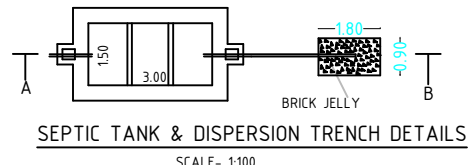
SEPTIC TANK & DISPERSION TRENCH DETAILS SCALE- 1:100
