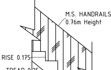
STAIRCASE DETAILS SCALE- 1:20
