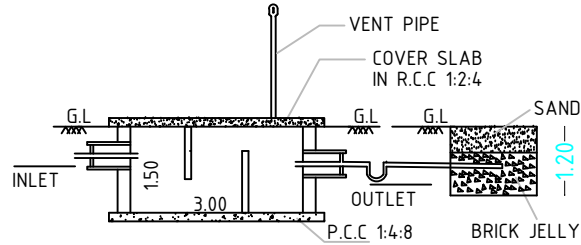
SECTION-AB
